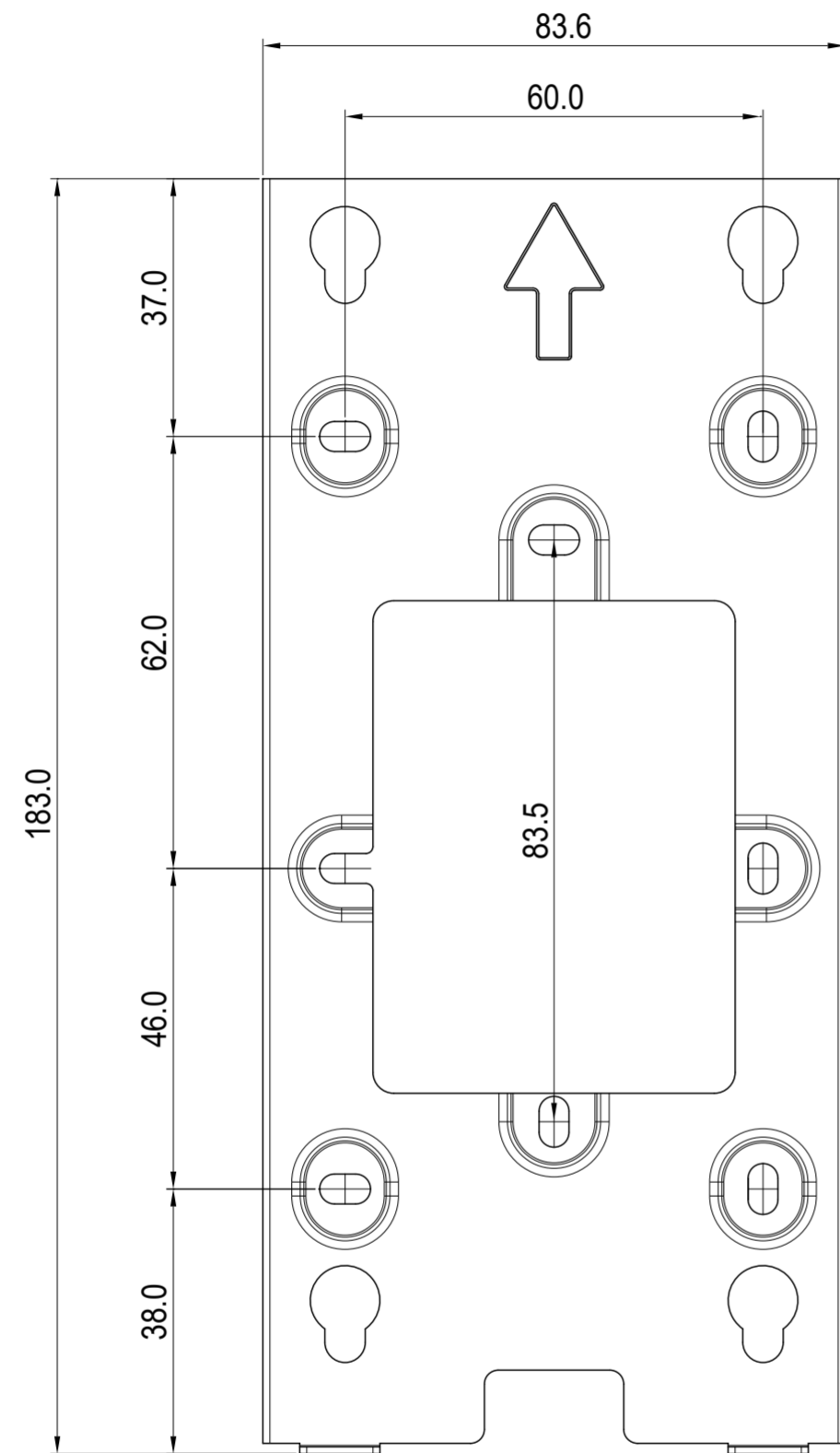
1 FRONT VIEW
